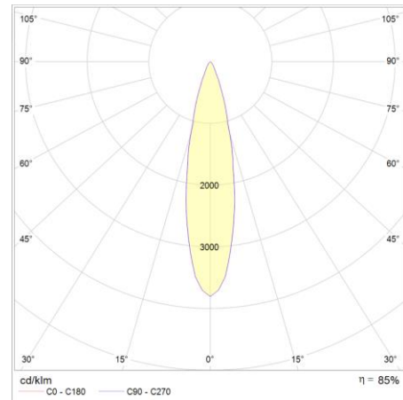
POLAR DIAGRAM 38°
