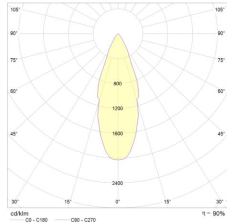
POLAR DIAGRAM 38°
