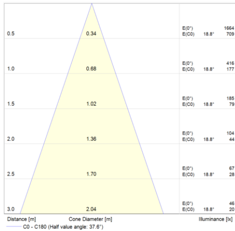
CONIC DIAGRAM 38°
