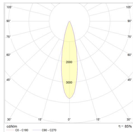
POLAR DIAGRAM 23°
