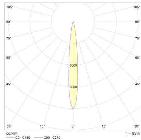
POLAR DIAGRAM 15°
