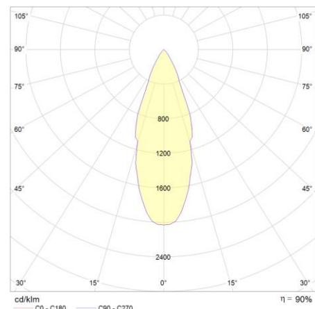
POLAR DIAGRAM 38°
