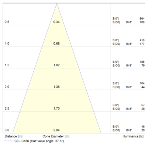
CONIC DIAGRAM 38°
