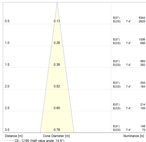
CONIC DIAGRAM 15°
